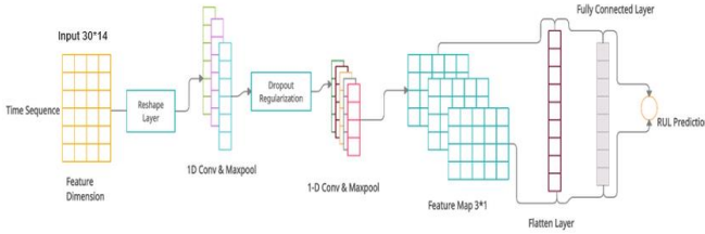
Figure 10. CNN Structure
